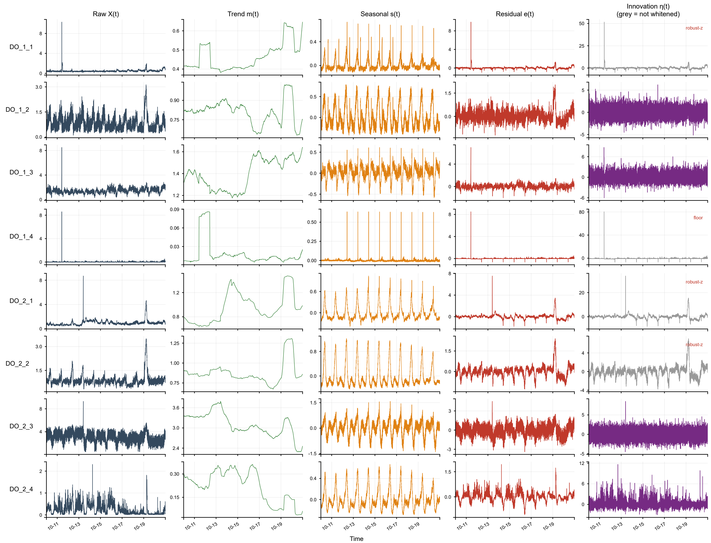
DO channels (both trains) — trend/seasonal/residual/innovation grid [2025-10-10~2025-10-20]
